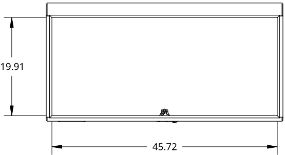
FLUSH OPENING LID OPTION (SHOWN) NOT FLUSH OPENING LID OPTION
